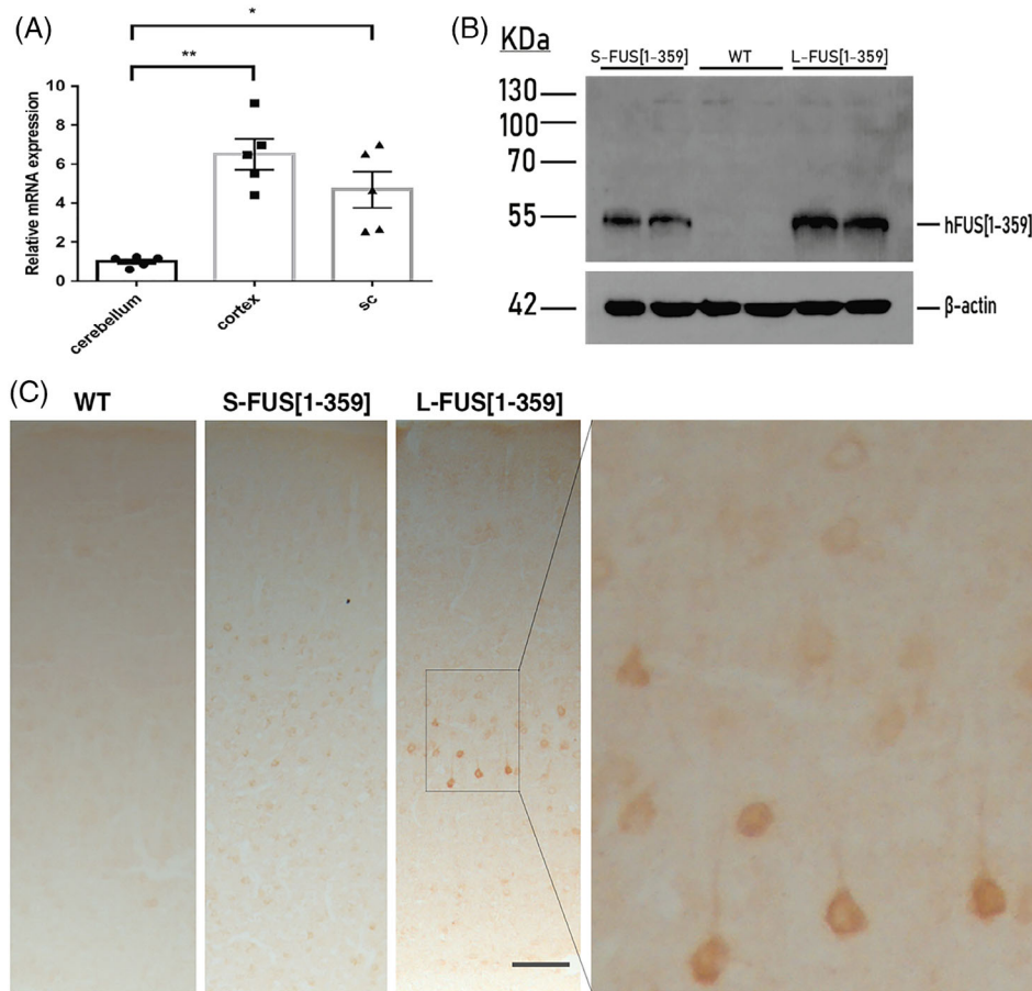
FIGURE 1 Expression of C-terminally truncated form of human FUS in the nervous system of L-FUS [1-359] mice. A, Relative levels of expression of transgenically expressed human FUS mRNA in the brain regions of ageing L-FUS[1-359] mice assessed by real-time qRT-PCR with primers specific for human FUS mRNA. Total RNA samples from five ageing (average age 299 days) homozygous L-FUS[1-359] male mice were analysed in triplicates (Kruskal-Wallis analysis of variance with Dunn's multiple comparisons test, **P < .01 , *P < .05 ). B, Western blot analysis of total protein samples extracted from the cortex of 2-month old hemizygous L-FUS[1-359], S-FUS [1-359] and wild type (WT) mice with antibody specific to human FUS. For loading control the same membrane was re-probed with anti-beta-actin antibody. C, Immunostaining of histological sections through the frontal cortex of L-FUS[1-359], S-FUS [1-359] and WT mice with antibody specific to human FUS. Scale bar, 100 \mu m
