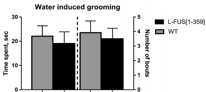
FIGURE 3 Water induced grooming test. Analysis of induced self-grooming in mice shows no significant changes in grooming behaviour between L-FUS[1-359] and wild type animals in the grooming time ( U = 57 , P = .4 ) and in the number of grooming bouts ( U = 63 , P = .6 ). N = 12 for both groups
