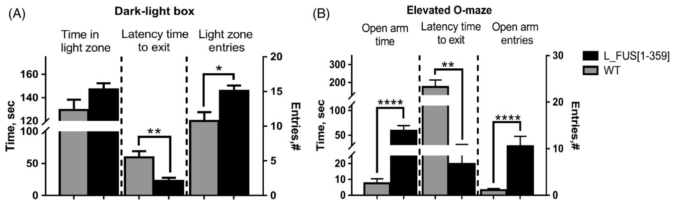
FIGURE 2 Behaviour tests for anxiety. A, In the light dark box test, transgenic L-FUS[1-359] mice display only a tendency to spent longer time in the light compartment ( U = 42 , P = .08 ) as compared with control WT mice. However, there was a significant reduction in the latency to first exit to the light compartment in L-FUS[1-359] mouse group ( U = 21 , P < .01 ). L-FUS[1-359] animals also have a significantly increased number of exits to the light compartment compared with control animals ( U = 32 , P < .05 ). B, In the elevated O-maze test L-FUS[1-359] mice displayed dramatically increased time spent in the open arm ( U = 7 , P < .0001 ) and the number of entries to the open arm ( U = 5 , P < .0001 ), as well as decreased latency to first exit to the open arm ( U = 22 , P < .01 ) compared with control WT animals. N = 12 for both groups
