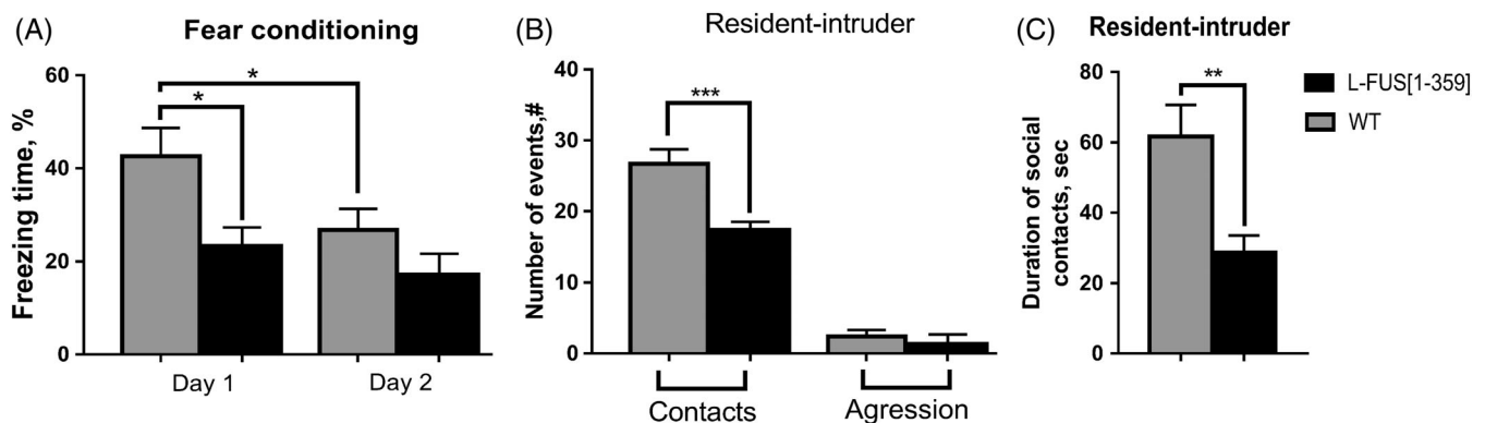
FIGURE 4 Analysis of memory and social function. A, In the contextual post-training fear-conditioning test, L-FUS[1-359] animals spent significantly lower time freezing than control animals ( U = 33.5 , P < .05 ). No significant differences between groups in the duration of freezing behaviour were observed in the test for extinguishing of contextual fear conditioning ( P = .09 ). Wild type mice show significant decrease in the time spent freezing 48 hours after the initial training compared with 24-hour post-training because, suggesting that mice have retrained in the post-training session ( U = 36 , P < .05 ). B, Analysis of social behaviour in resident-intruder test show that L-FUS[1-359] mice show significantly less social interest ( U = 16 , P < .001 ) in exploring the intruder mice. Both L-FUS[1-359] and WT mice has not shown high level of aggression and violence. C, Analysis of the duration of social contacts in resident-intruder test also show that L-FUS[1-359] mice spent significantly less time ( U = 25 , P < .01 ) exploring intruder mice. N = 12 for both groups
